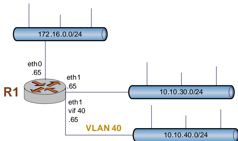
Figure 1-3 VLAN configuration
