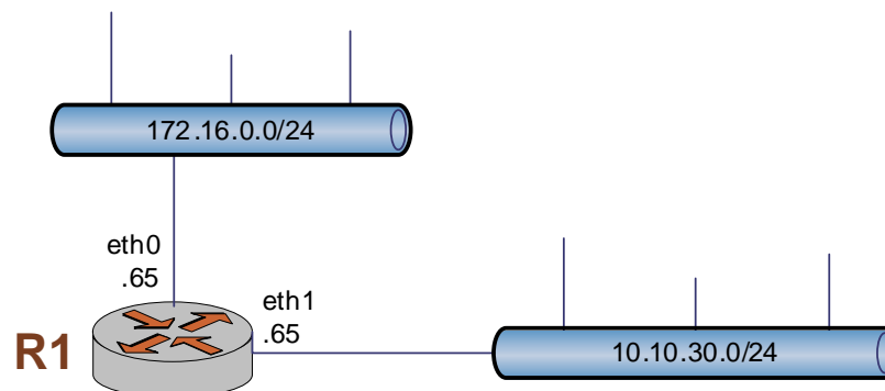
Figure 1-1 Basic Ethernet interface configuration
